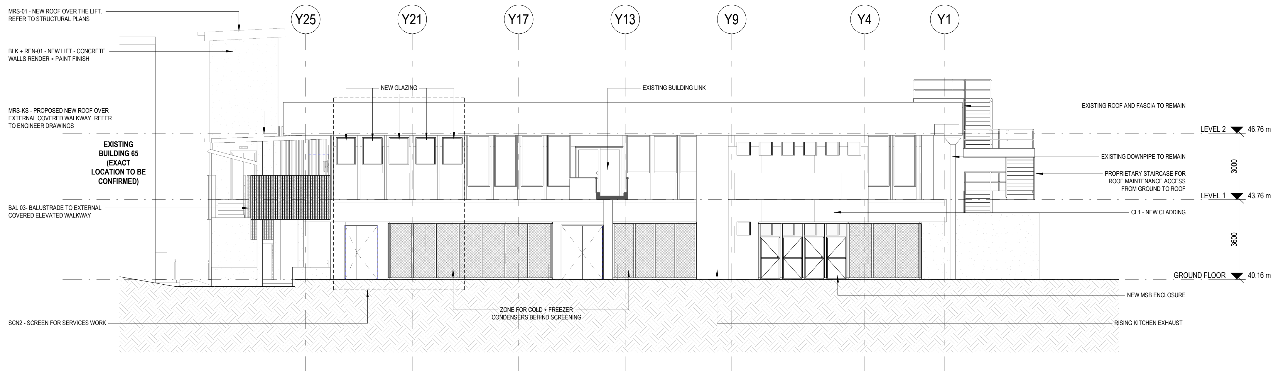
1 SOUTH ELEVATION - PROPOSED 21-01 1 : 100
