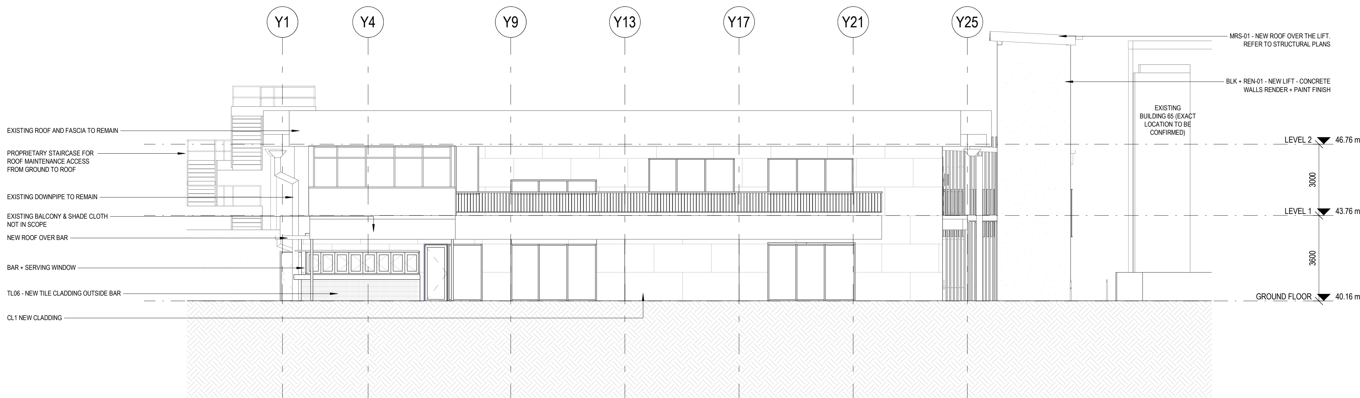
2 NORTH ELEVATION - PROPOSED 21-01 1 : 100
